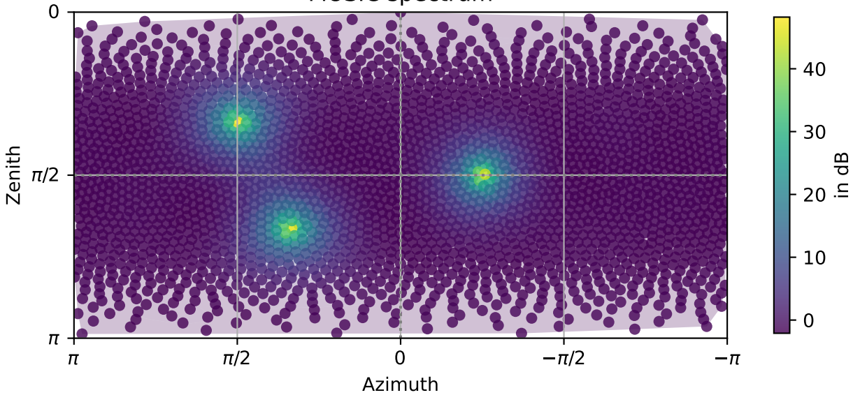
MUSIC spectrum
